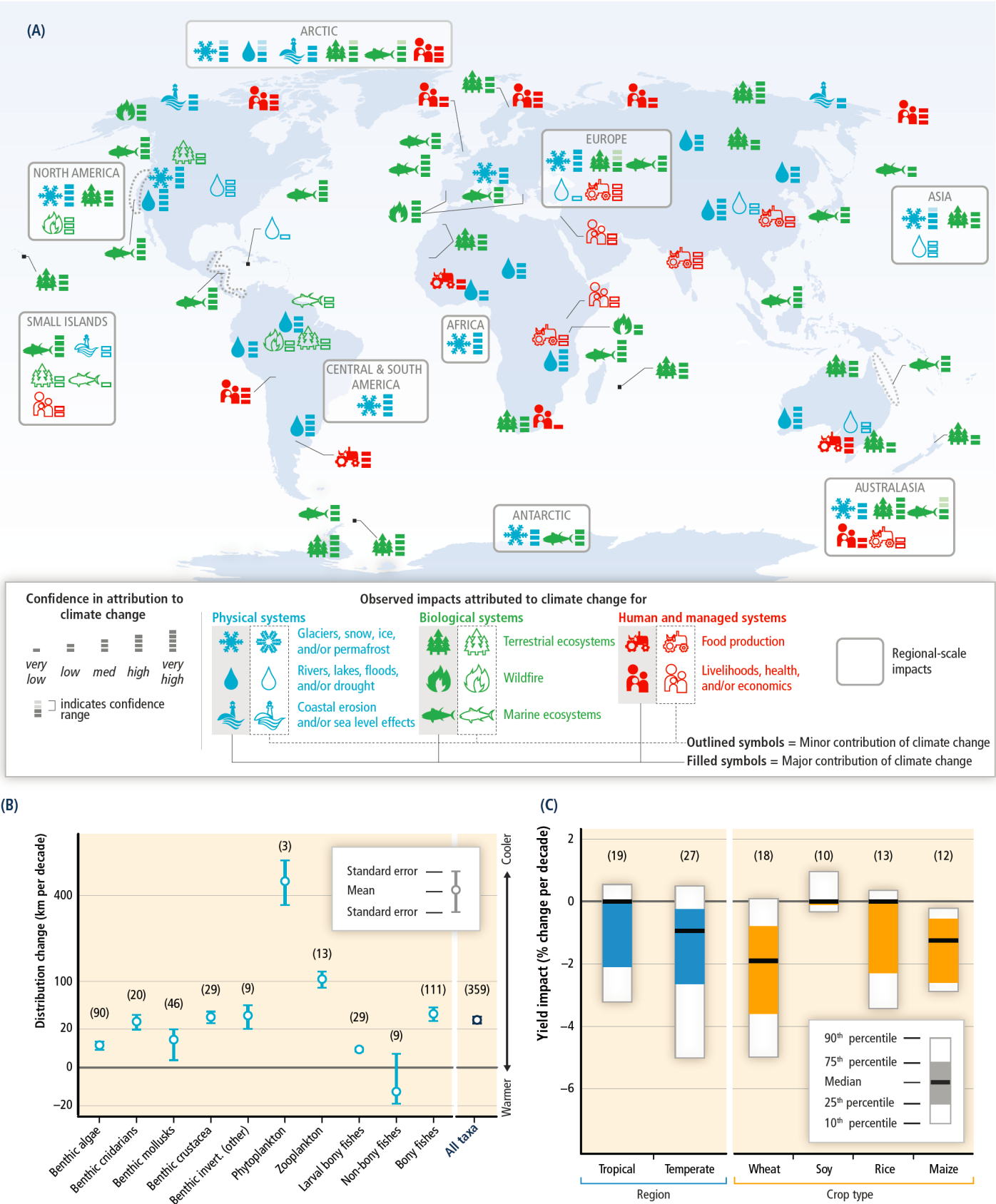
Figure SPM.2.
