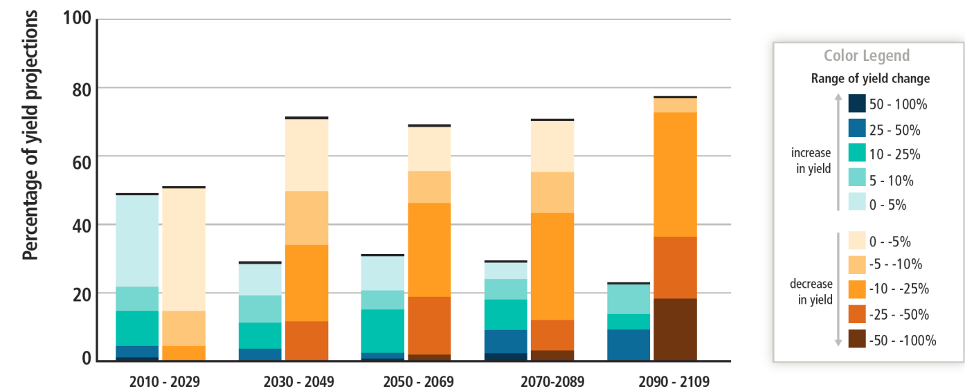
Figure SPM.7.
