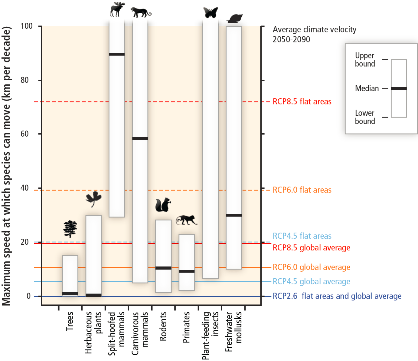
Figure SPM.5.
