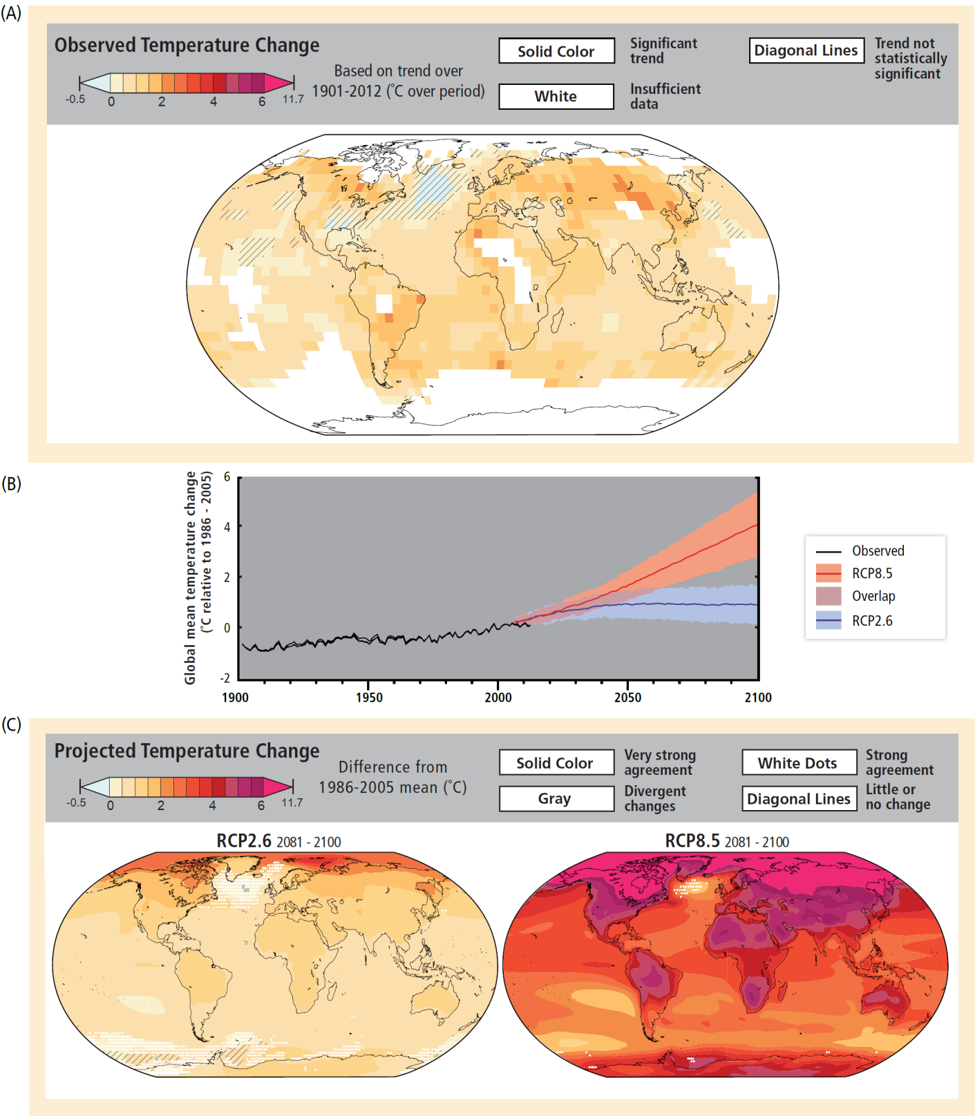
Figure SPM.4.
