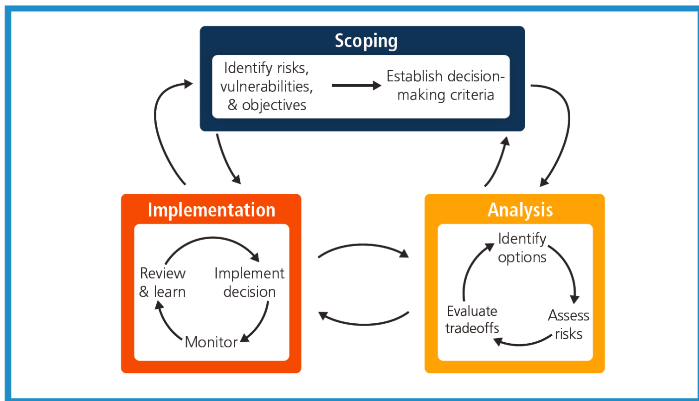
Figure SPM.3.
