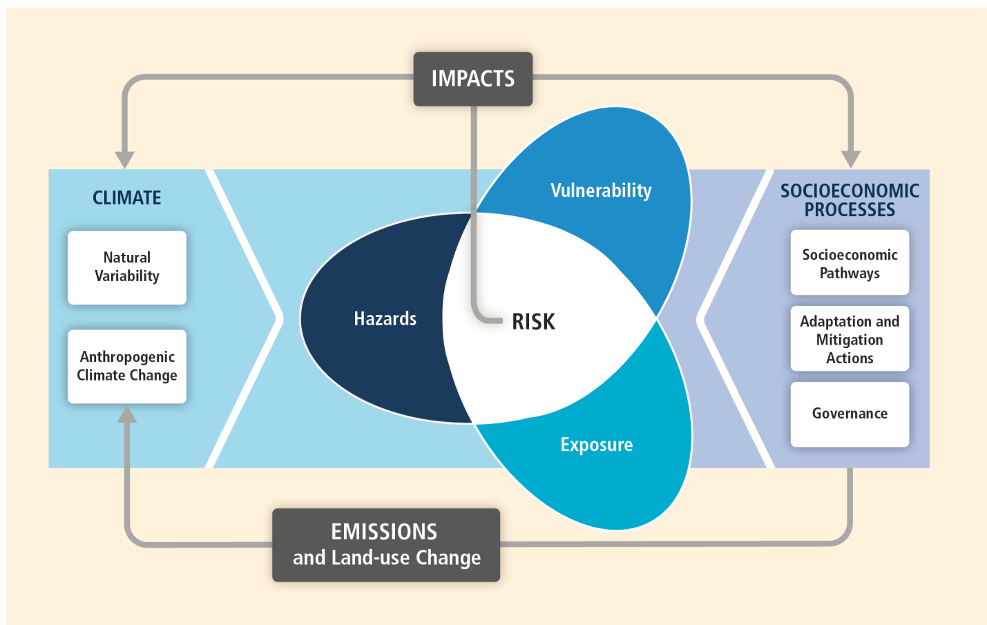
Figure SPM.1.
